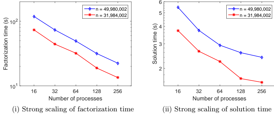
FIG. 6.2. Strong scaling tests with PRSMF for two discretized matrices from the 2D linear elasticity equation.
