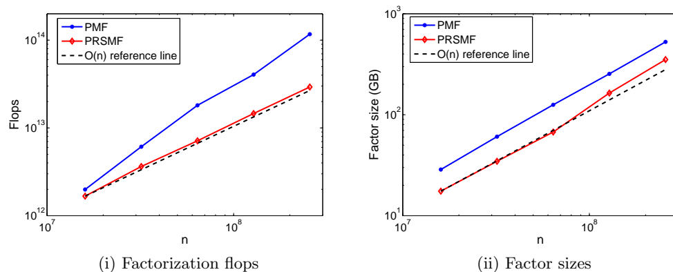
FIG. 6.1. Factorization flops and factor sizes in Table 6.1 for discretized matrices from the 2D Poisson's equation.
