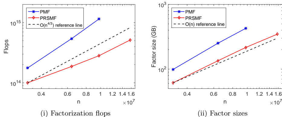
FIG. 6.4. Factorization flops and factor sizes in Table 6.3 for discretized matrices from the 3D Helmholtz equation.
