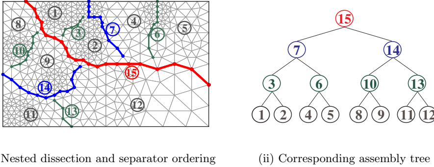
FIG. 2.1. Nested dissection of a mesh and the corresponding assembly tree, where the mesh illustration is based on Meshpart [13].
