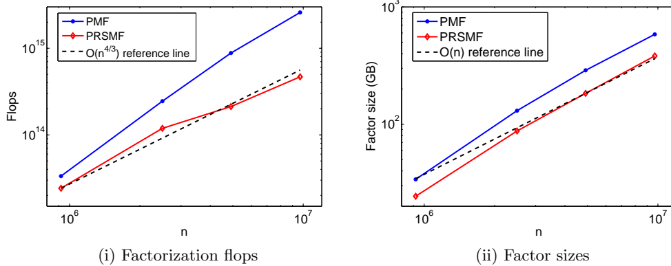
FIG. 6.6. Factorization flops and factor sizes in Table 6.4 for discretized matrices from the 3D elastic wave equation.
