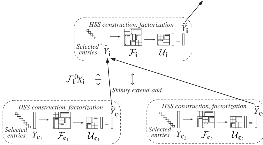
FIG. 3.1. Illustration of the randomized structured multifrontal (RSMF) method in [31]. For simplicity, only a symmetric version is used for the illustration purpose.
