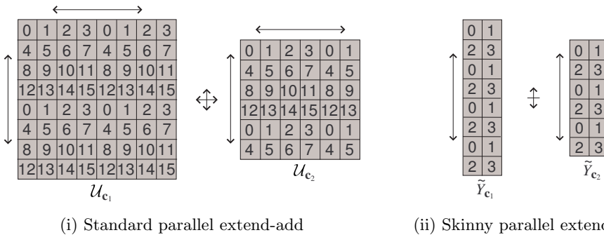
FIG. 4.4. Parallel skinny extend-add operation as compared with the standard dense one, where the matrices are stored on a process grid. The skinny one deals with much less data and also needs only row permutations.
