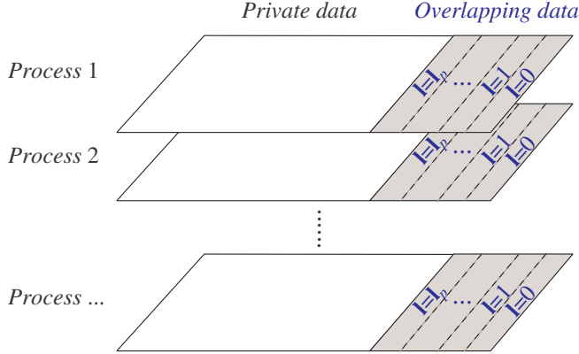
FIG. 4.2. Storage scheme for the sparse matrix A . Below the parallel level \mathbf{l}_p , each process stores a private portion of A . Above \mathbf{l}_p , each process stores overlapping data associated with its accessible nodes at each level \mathbf{l} = 0, 1, \dots, \mathbf{l}_p .
