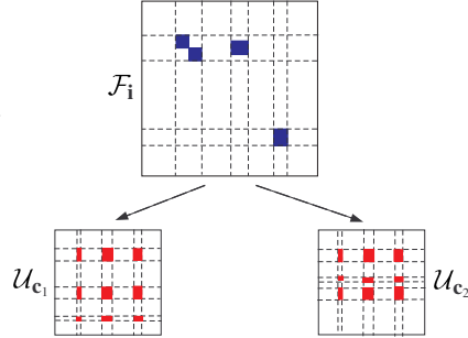
FIG. 4.5. Mapping the row and column index sets of selected entries of \mathcal{F}_i to those of \mathcal{U}_{c_1} and \mathcal{U}_{c_2} .
