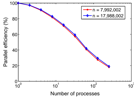
FIG. 6.3. Parallel efficiency of PRSMF for two discretized matrices from the 2D linear elasticity equation.
