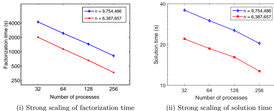
FIG. 6.5. Strong scaling tests with PRSMF for two discretized matrices from the 3D Helmholtz equation.
