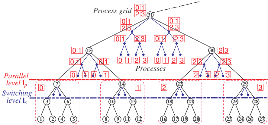
FIG. 4.1. Static mapping model for our parallel randomized structured multifrontal (PRSMF) method, where the outer-layer tree is the assembly tree, and the inner-layer trees are HSS trees.
