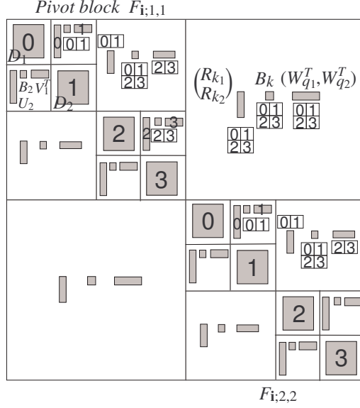
FIG. 4.3. Distributed memory storage for an HSS form frontal matrix \mathcal{F}_i given 4 processes, where k_1, k_2 are the children of k (root of the HSS tree T_1 for \mathcal{F}_{i;1,1} ) and q_1, q_2 are the children of q (root of the HSS tree T_2 for \mathcal{F}_{i;2,2} ). See the inner layer tree associated with node i = 31 in Figure 4.1.
